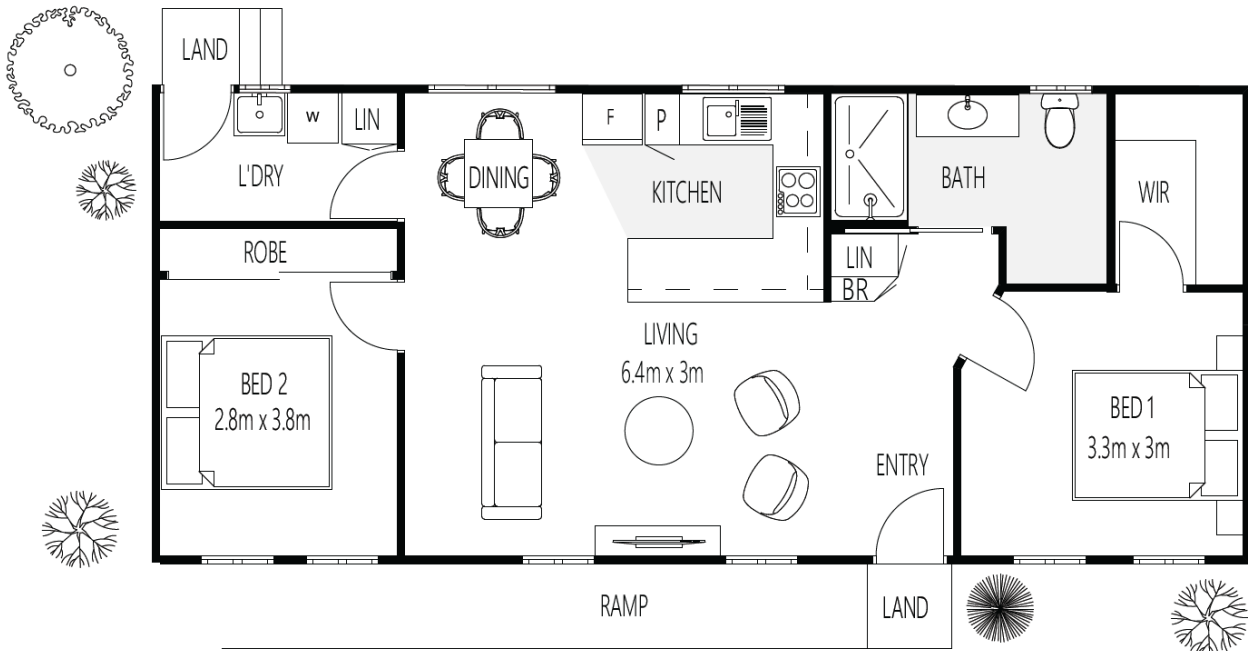
LYNBROOK – 12.9m x 5.6m / 72.24m 2
